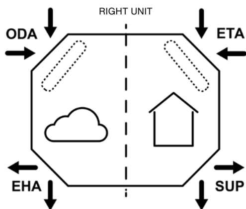
Supply and extract air to right
